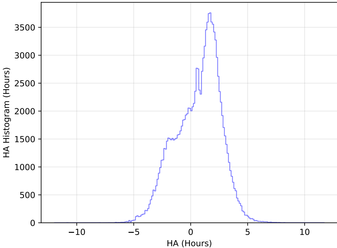
ddf_acor_sf10_lsf30_lsr20_v3.4_10yrs WFD u band: HA Histogram
