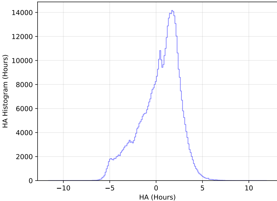
ddf_acor_sf10_lsf30_lsr20_v3.4_10yrs WFD r band: HA Histogram
