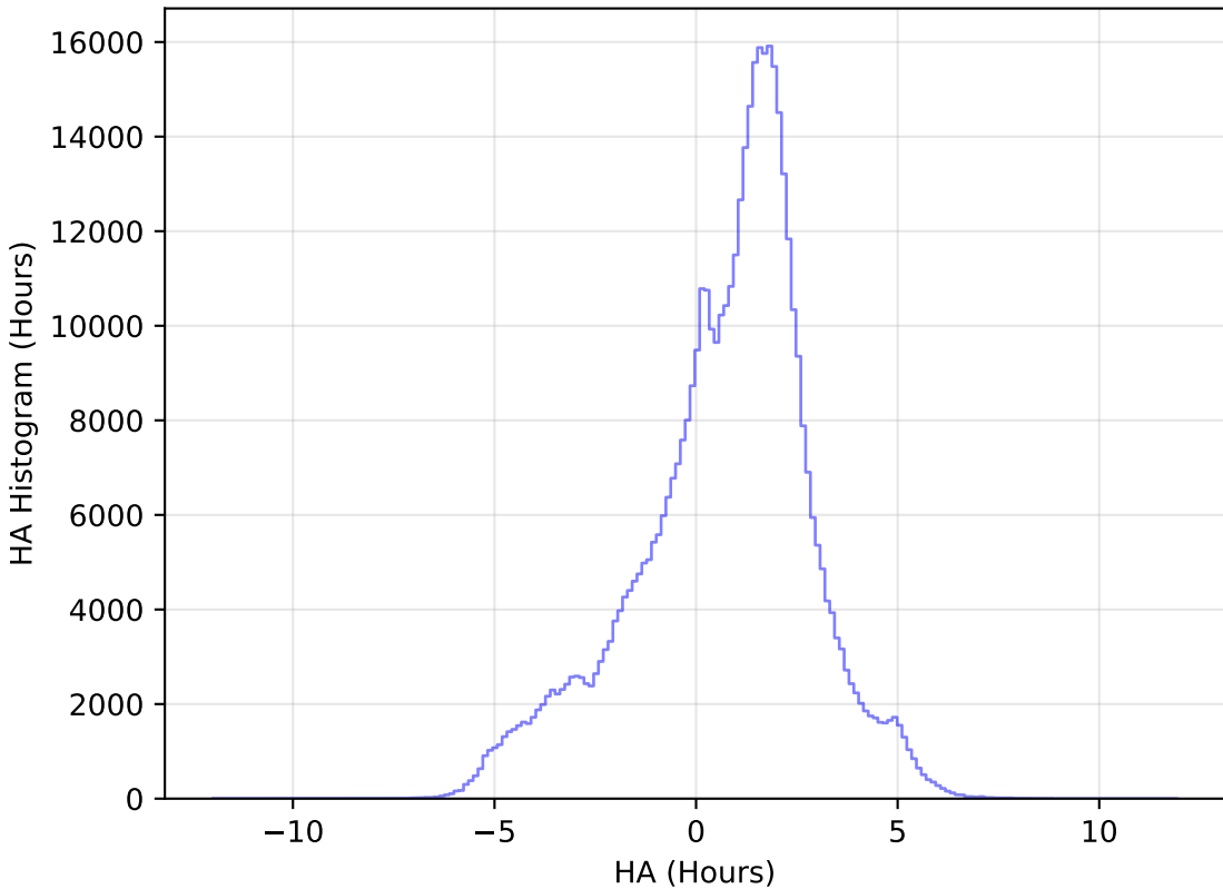
ddf_acor_sf10_lsf30_lsr20_v3.4_10yrs WFD i band: HA Histogram
