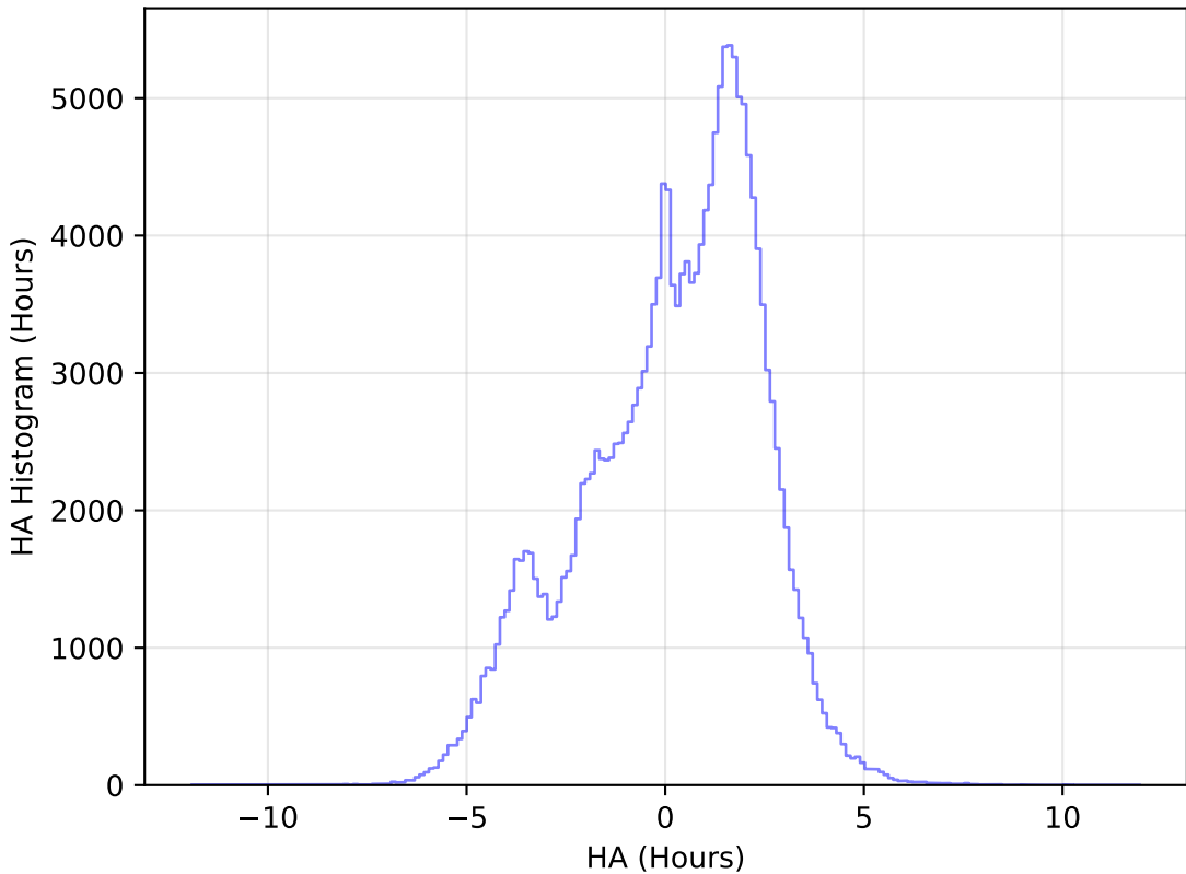
ddf_acor_sf10_lsf30_lsr20_v3.4_10yrs WFD g band: HA Histogram
