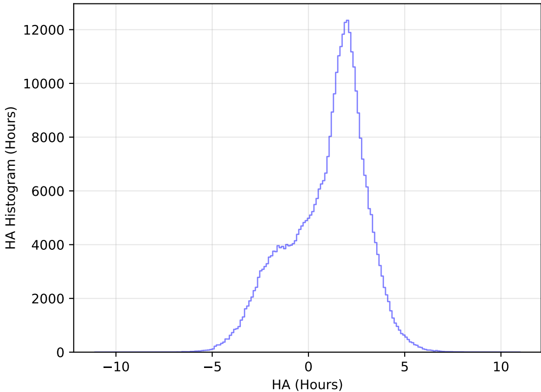
ddf_acor_sf10_lsf30_lsr20_v3.4_10yrs All sky y band: HA Histogram
