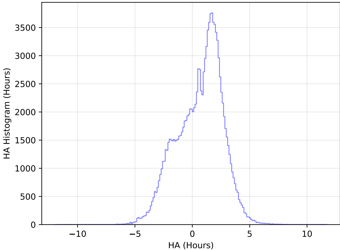
ddf_acor_sf10_lsf30_lsr20_v3.4_10yrs All sky u band: HA Histogram
