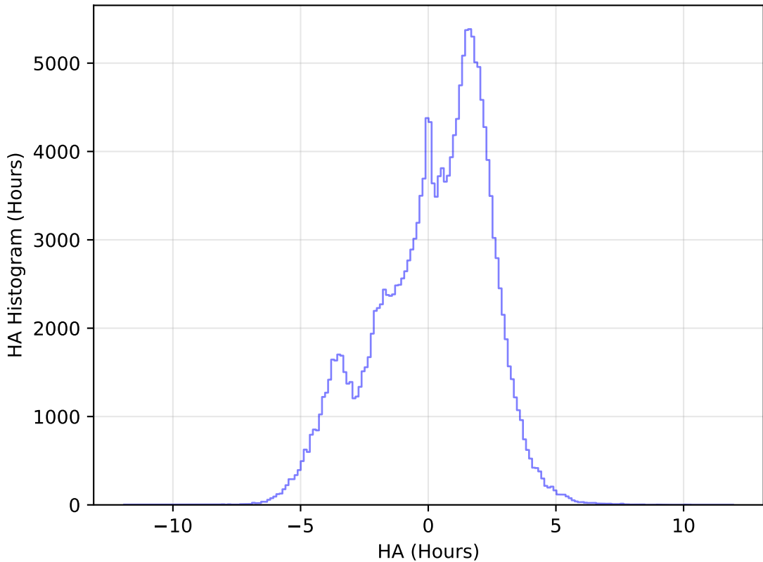
ddf_acor_sf10_lsf30_lsr20_v3.4_10yrs All sky g band: HA Histogram
