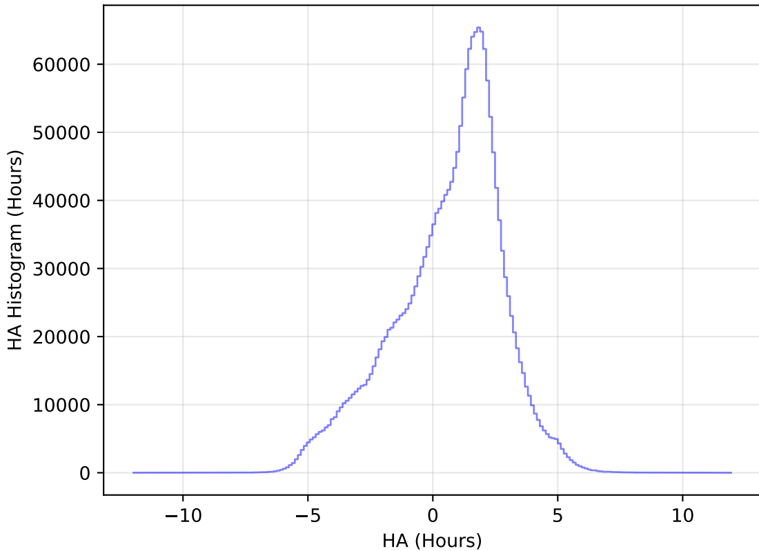
ddf_acor_sf10_lsf30_lsr20_v3.4_10yrs All sky all bands: HA Histogram
