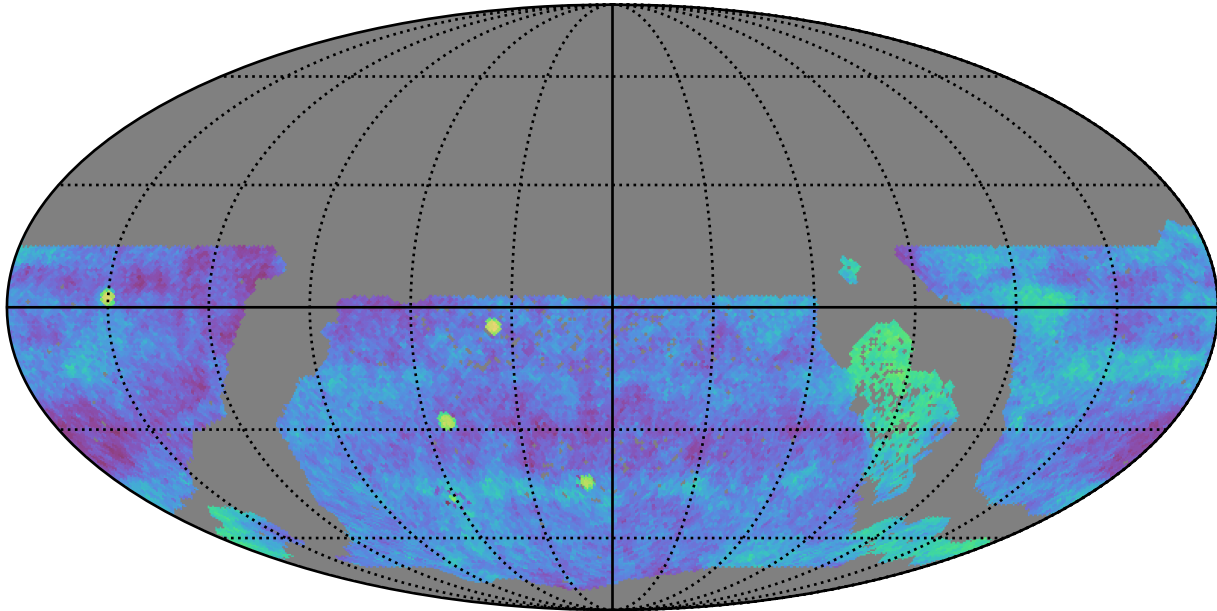
ddf_acor_sf10_lsf30_lsr20_v3.4_10yrs gri WFD: Fraction of visits in pairs (20-90 min)
