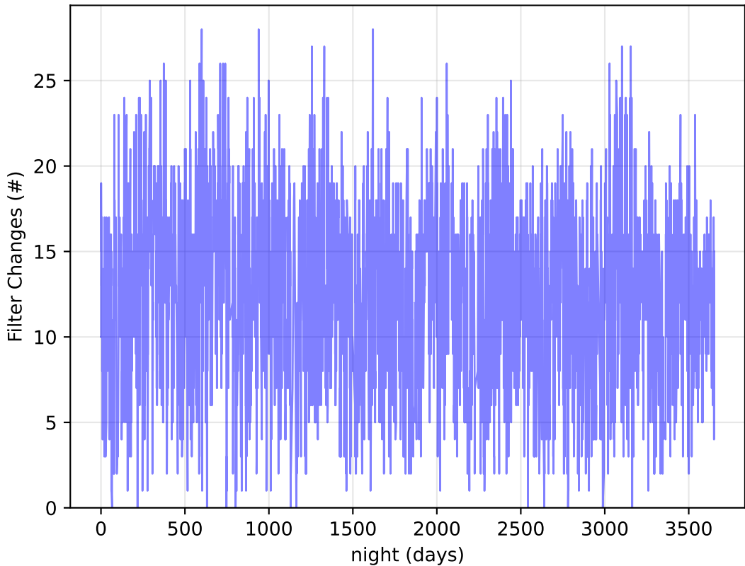
ddf_acor_sf10_lsf30_lsr20_v3.4_10yrs Per Night: Filter Changes
