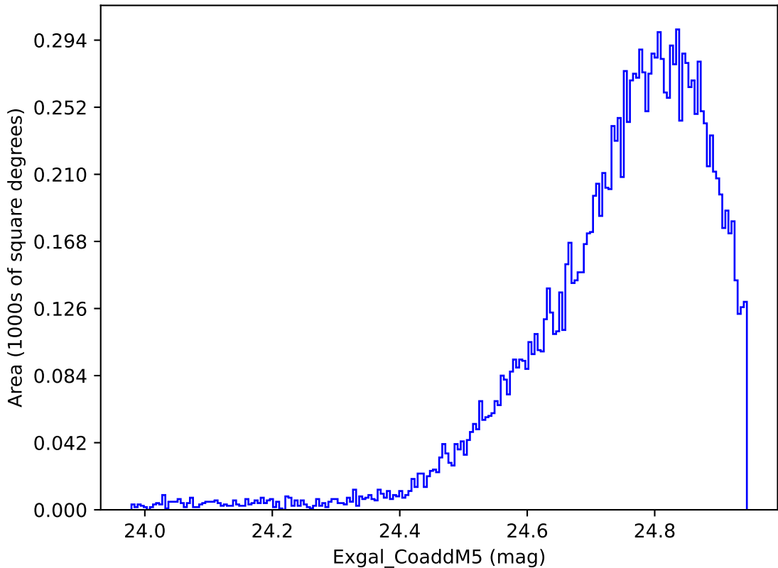
ddf_acor_sf10_lsf30_lsr20_v3.4_10yrs WFD y band: Exgal_CoaddM5
