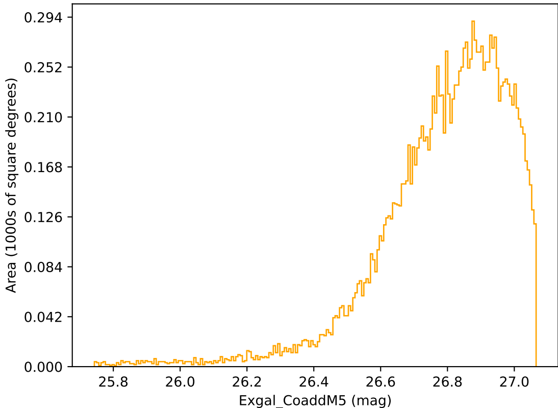
ddf_acor_sf10_lsf30_lsr20_v3.4_10yrs WFD r band: Exgal_CoaddM5
