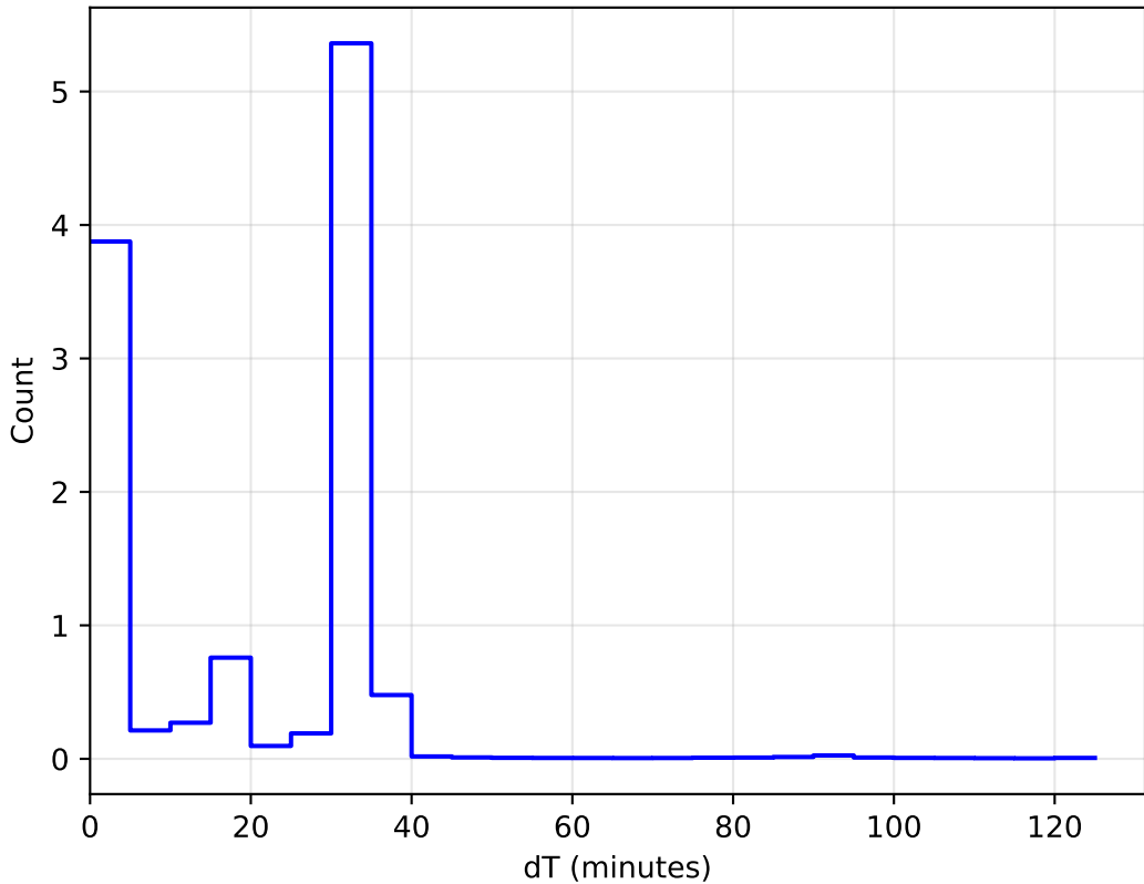
ddf_acor_sf10_lsf30_lsr20_v3.4_10yrs WFD: DeltaT Histogram 1e6
