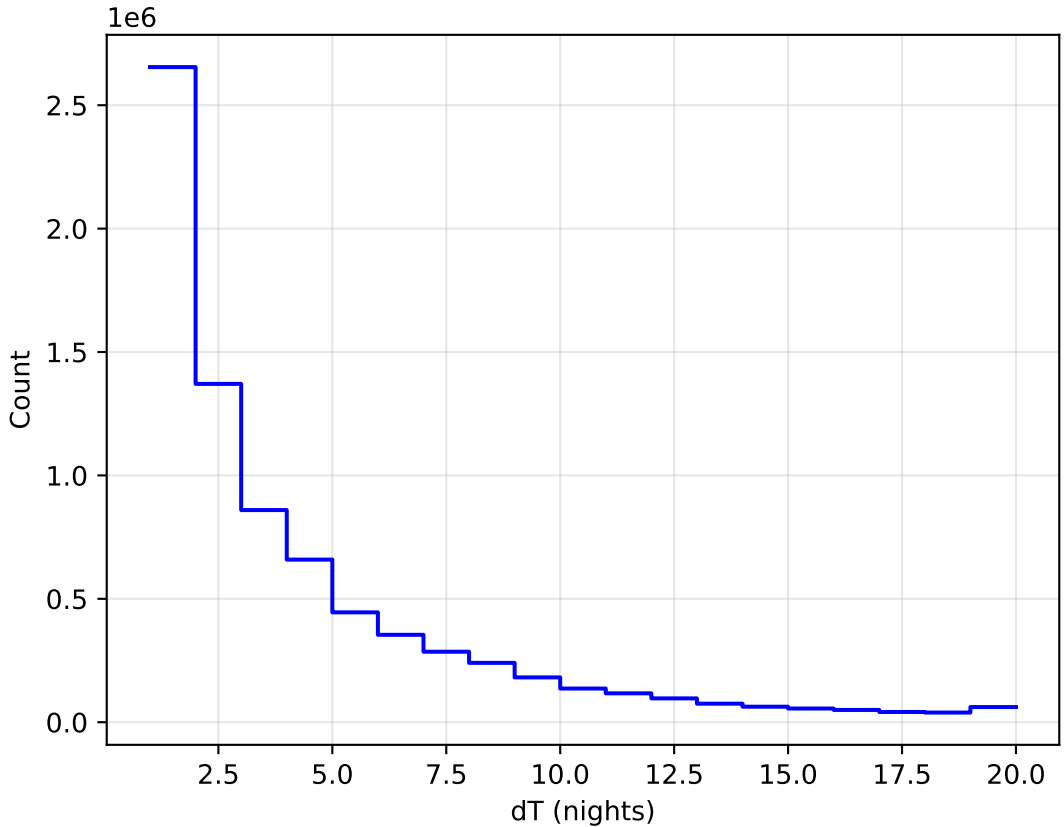
ddf_acor_sf10_lsf30_lsr20_v3.4_10yrs WFD all bands: DeltaNight Histogram
