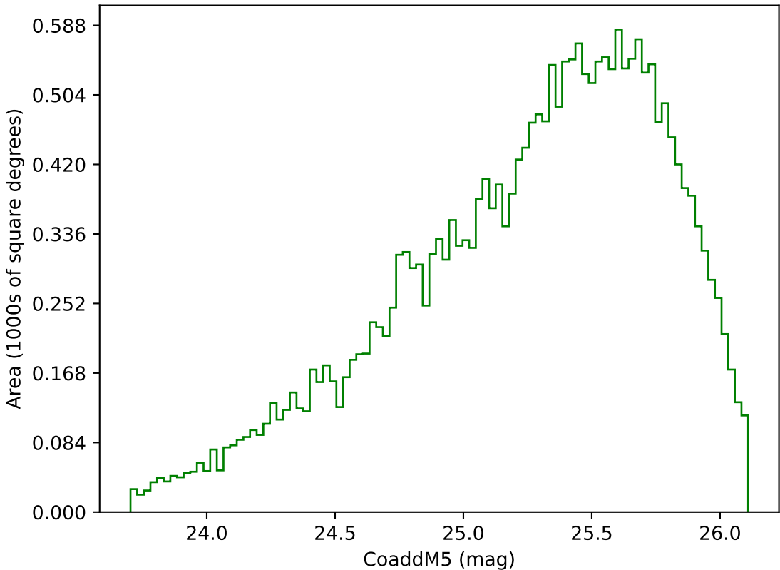
ddf_acor_sf10_lsf30_lsr20_v3.4_10yrs Yr 3-4 g band: CoaddM5
