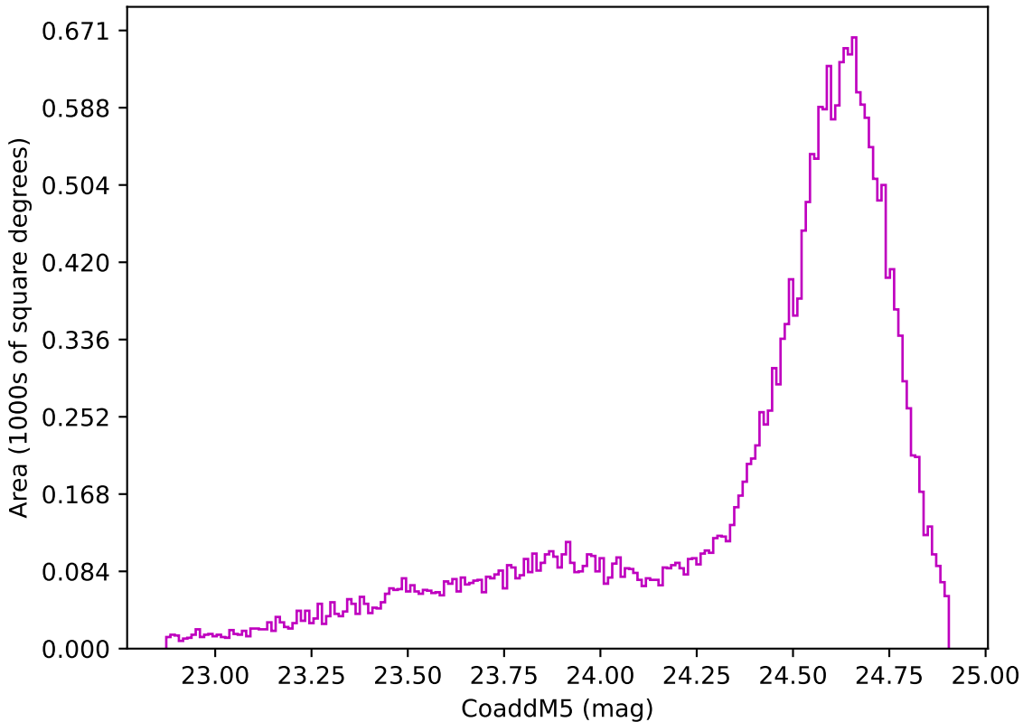
ddf_acor_sf10_lsf30_lsr20_v3.4_10yrs Yr 1 z band: CoaddM5
