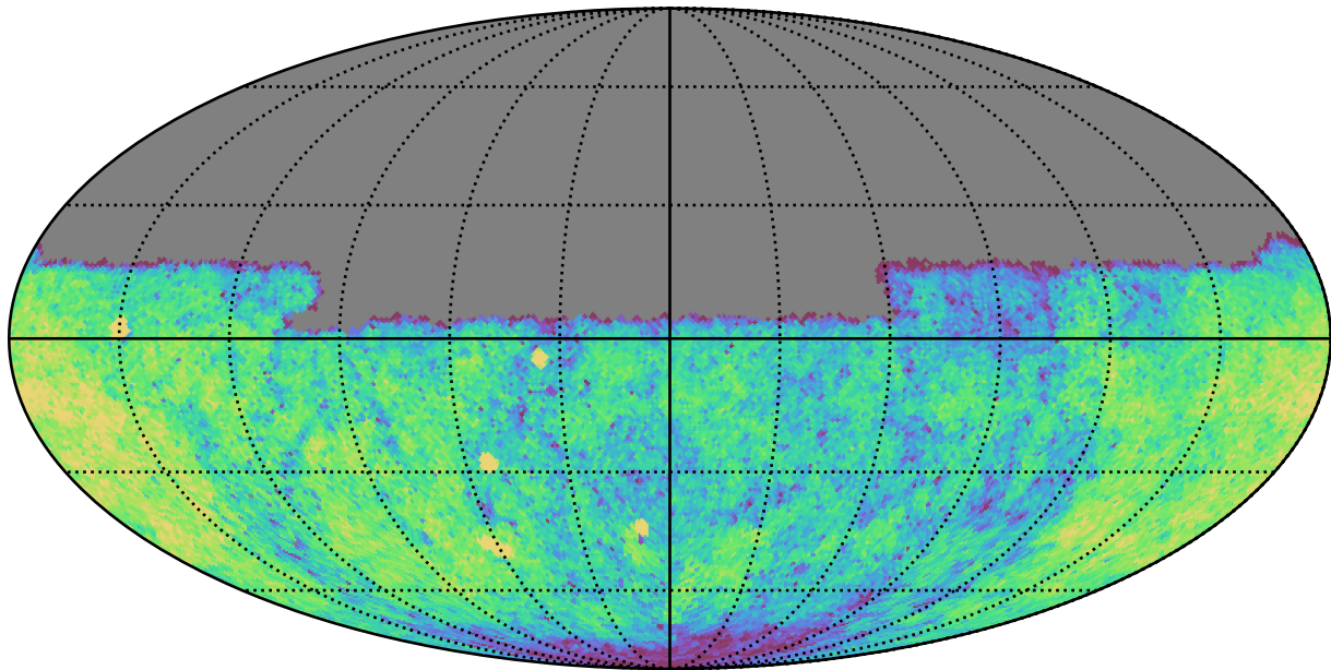
ddf_acor_sf10_lsf30_lsr20_v3.4_10yrs Yr 1 u band: CoaddM5
