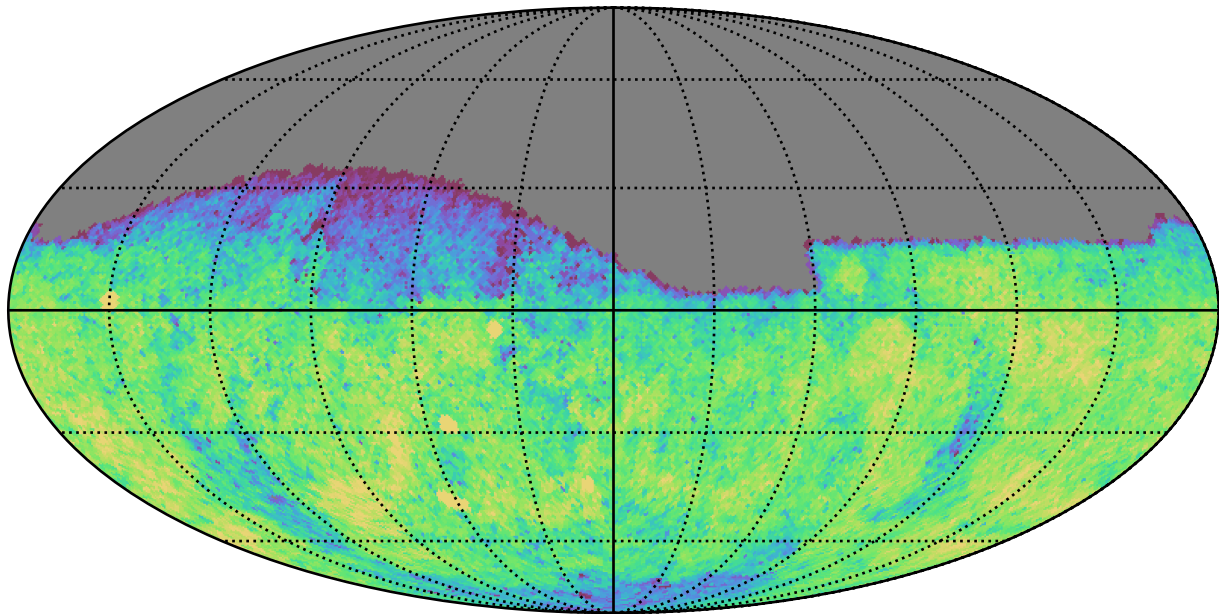
ddf_acor_sf10_lsf30_lsr20_v3.4_10yrs Yr 1 g band: CoaddM5
