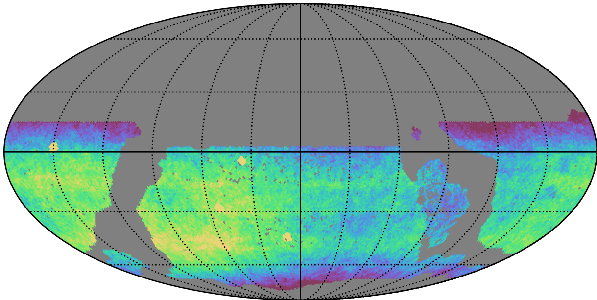
ddf_acor_sf10_lsf30_lsr20_v3.4_10yrs WFD z band: CoaddM5
