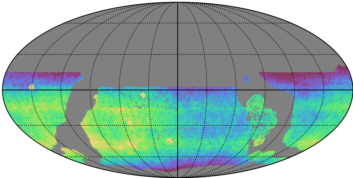
ddf_acor_sf10_lsf30_lsr20_v3.4_10yrs WFD r band: CoaddM5
