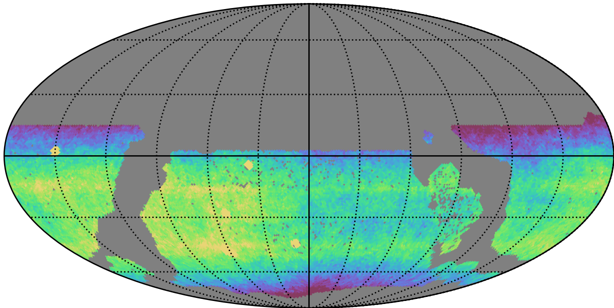
ddf_acor_sf10_lsf30_lsr20_v3.4_10yrs WFD i band: CoaddM5
