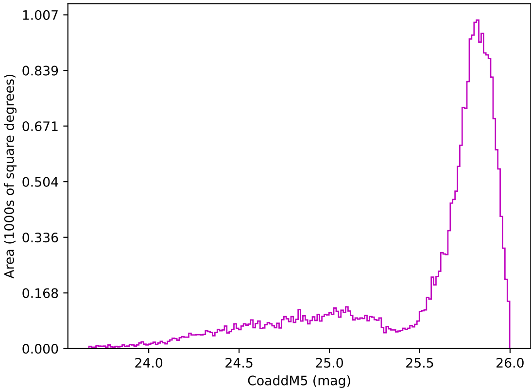
ddf_acor_sf10_lsf30_lsr20_v3.4_10yrs All sky z band: CoaddM5
