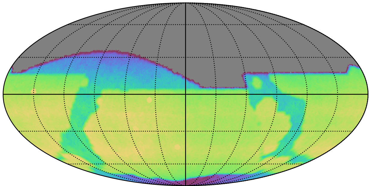
ddf_acor_sf10_lsf30_lsr20_v3.4_10yrs All sky r band: CoaddM5
