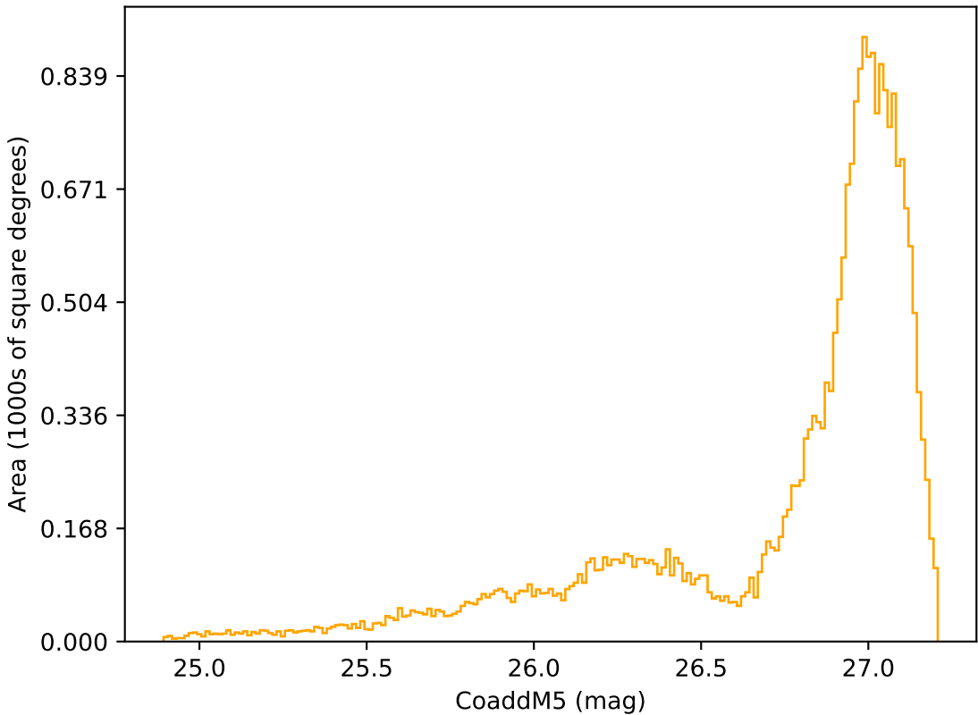
ddf_acor_sf10_lsf30_lsr20_v3.4_10yrs All sky r band: CoaddM5
