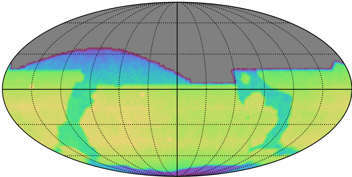
ddf_acor_sf10_lsf30_lsr20_v3.4_10yrs All sky i band: CoaddM5
