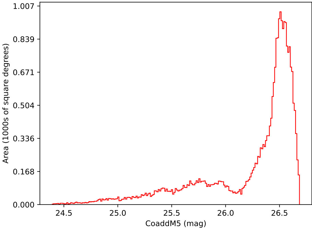
ddf_acor_sf10_lsf30_lsr20_v3.4_10yrs All sky i band: CoaddM5
