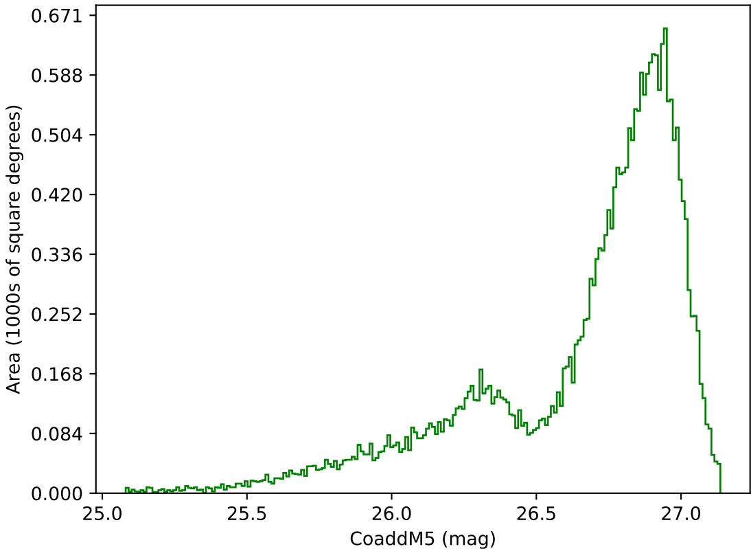
ddf_acor_sf10_lsf30_lsr20_v3.4_10yrs All sky g band: CoaddM5
