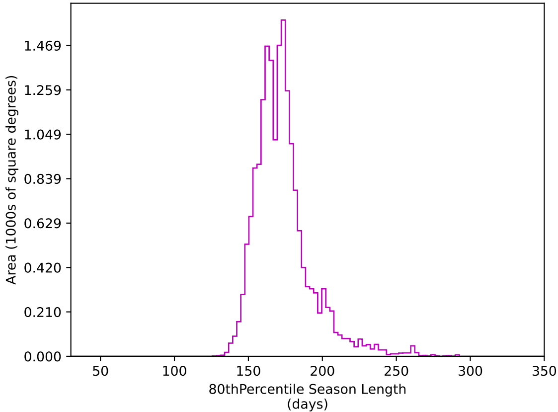
ddf_acor_sf10_lsf30_lsr20_v3.4_10yrs WFD z band: 80thPercentile Season Length
