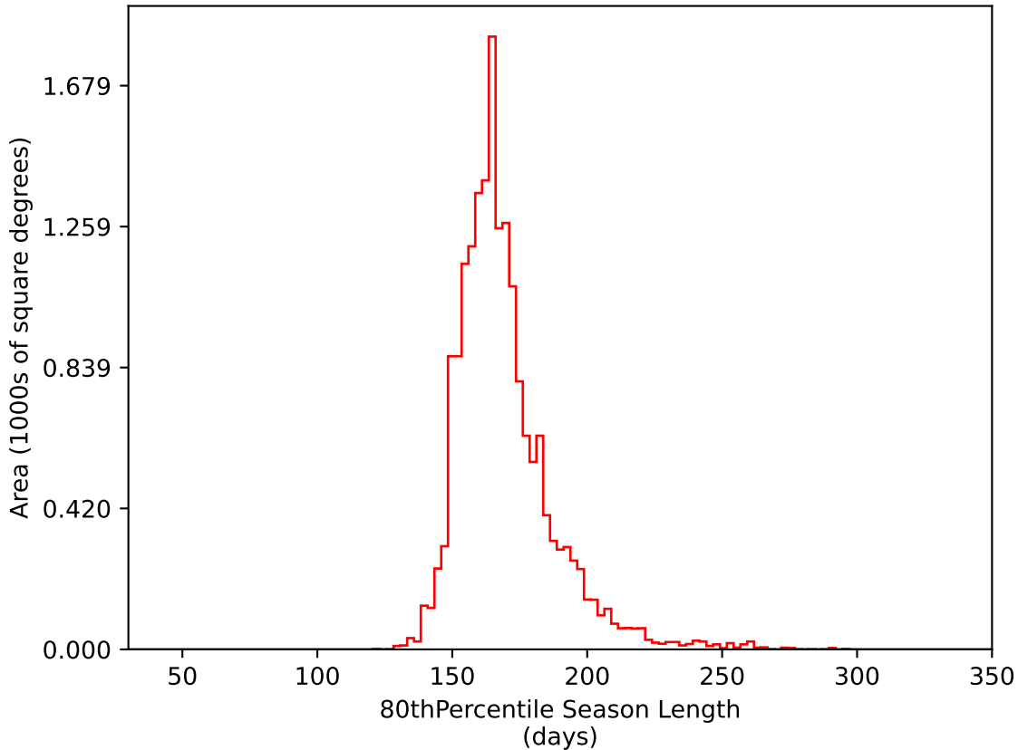
ddf_acor_sf10_lsf30_lsr20_v3.4_10yrs WFD i band: 80thPercentile Season Length
