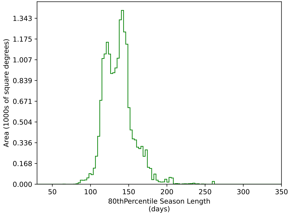
ddf_acor_sf10_lsf30_lsr20_v3.4_10yrs WFD g band: 80thPercentile Season Length
