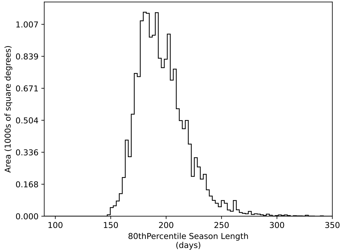
ddf_acor_sf10_lsf30_lsr20_v3.4_10yrs WFD all bands: 80thPercentile Season Length
