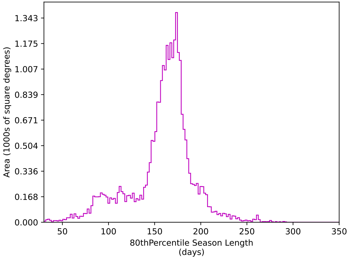
ddf_acor_sf10_lsf30_lsr20_v3.4_10yrs All sky z band: 80thPercentile Season Length
