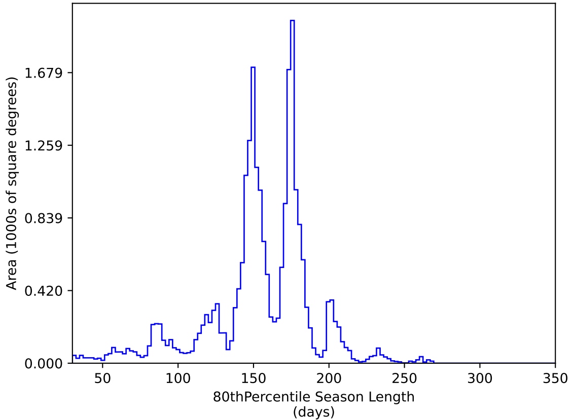
ddf_acor_sf10_ls30_lsr20_v3.4_10yrs All sky y band: 80thPercentile Season Length
