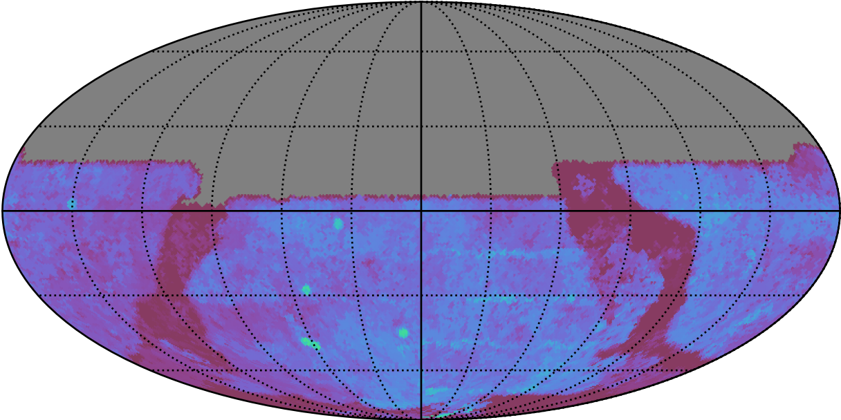
ddf_acor_sf10_lsf30_lsr20_v3.4_10yrs All sky u band: 80thPercentile Season Length
