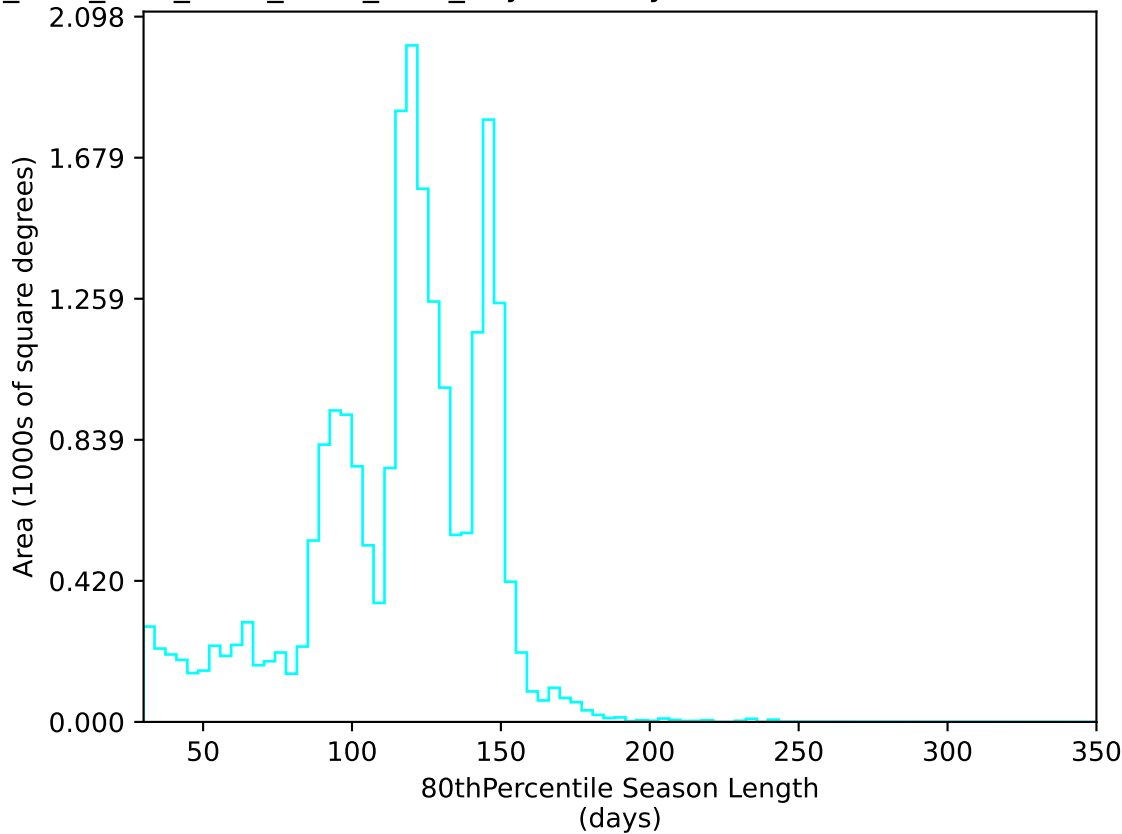
ddf_acor_sf10_lsf30_lsr20_v3.4_10yrs All sky u band: 80thPercentile Season Length
