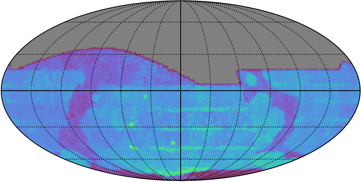
ddf_acor_sf10_lsf30_lsr20_v3.4_10yrs All sky r band: 80thPercentile Season Length
