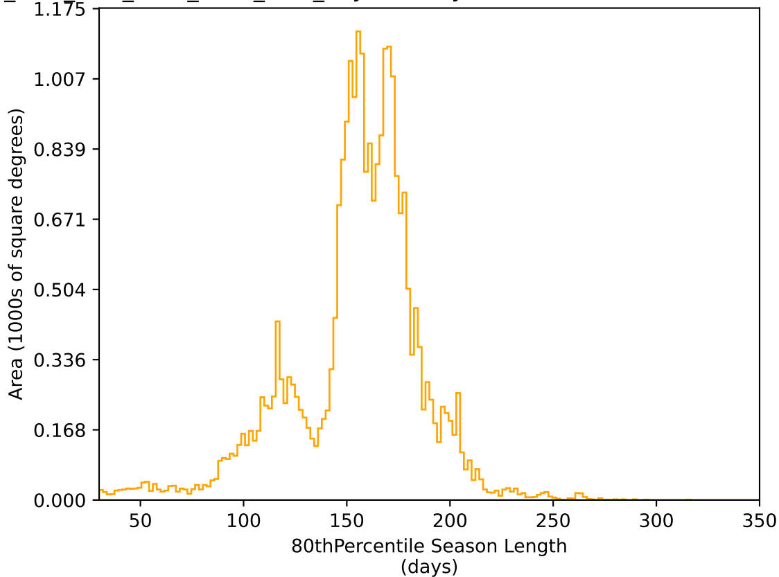
ddf_acor_sf10_lsf30_lsr20_v3.4_10yrs All sky r band: 80thPercentile Season Length
