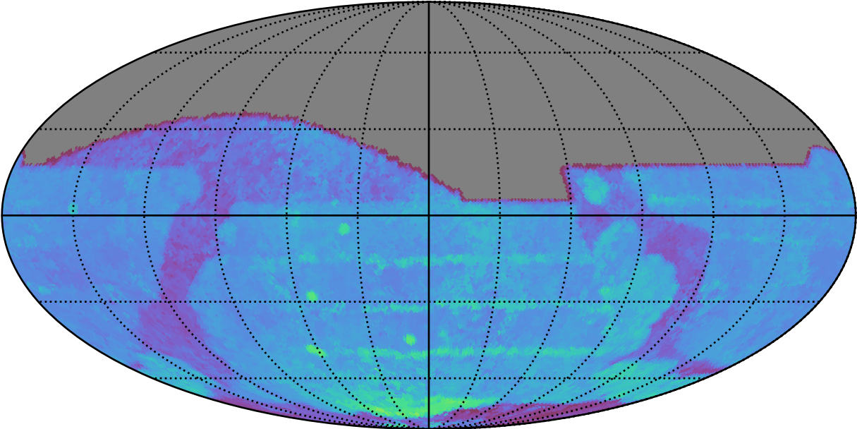
ddf_acor_sf10_lsf30_lsr20_v3.4_10yrs All sky i band: 80thPercentile Season Length
