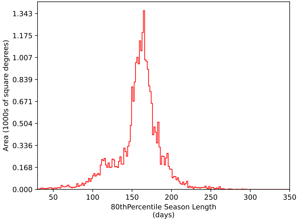
ddf_acor_sf10_lsf30_lsr20_v3.4_10yrs All sky i band: 80thPercentile Season Length
