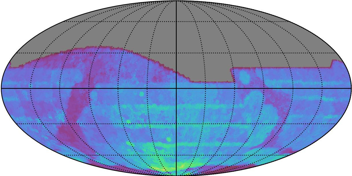
ddf_acor_sf10_lsf30_lsr20_v3.4_10yrs All sky all bands: 80thPercentile Season Length
