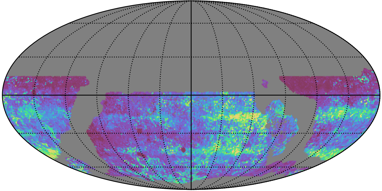
ddf_acor_sf10_lsf30_lsr20_v3.4_10yrs WFD zy bands: 75th Percentile Intranight Timespan
