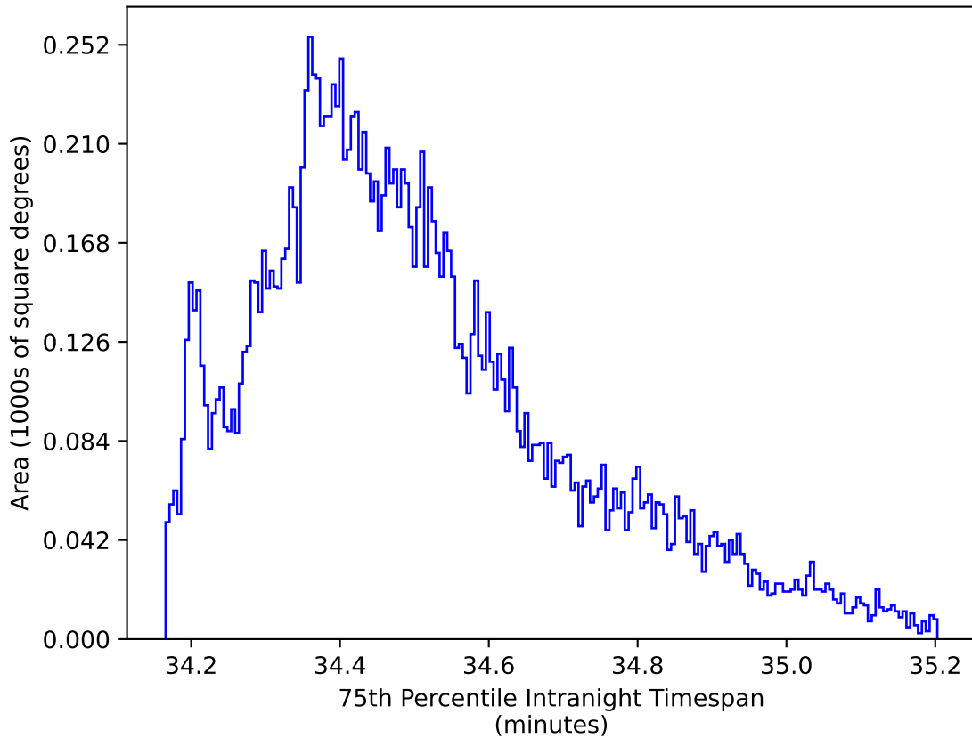
ddf_acor_sf10_lsf30_lsr20_v3.4_10yrs WFD zy bands: 75th Percentile Intranight Timespan
