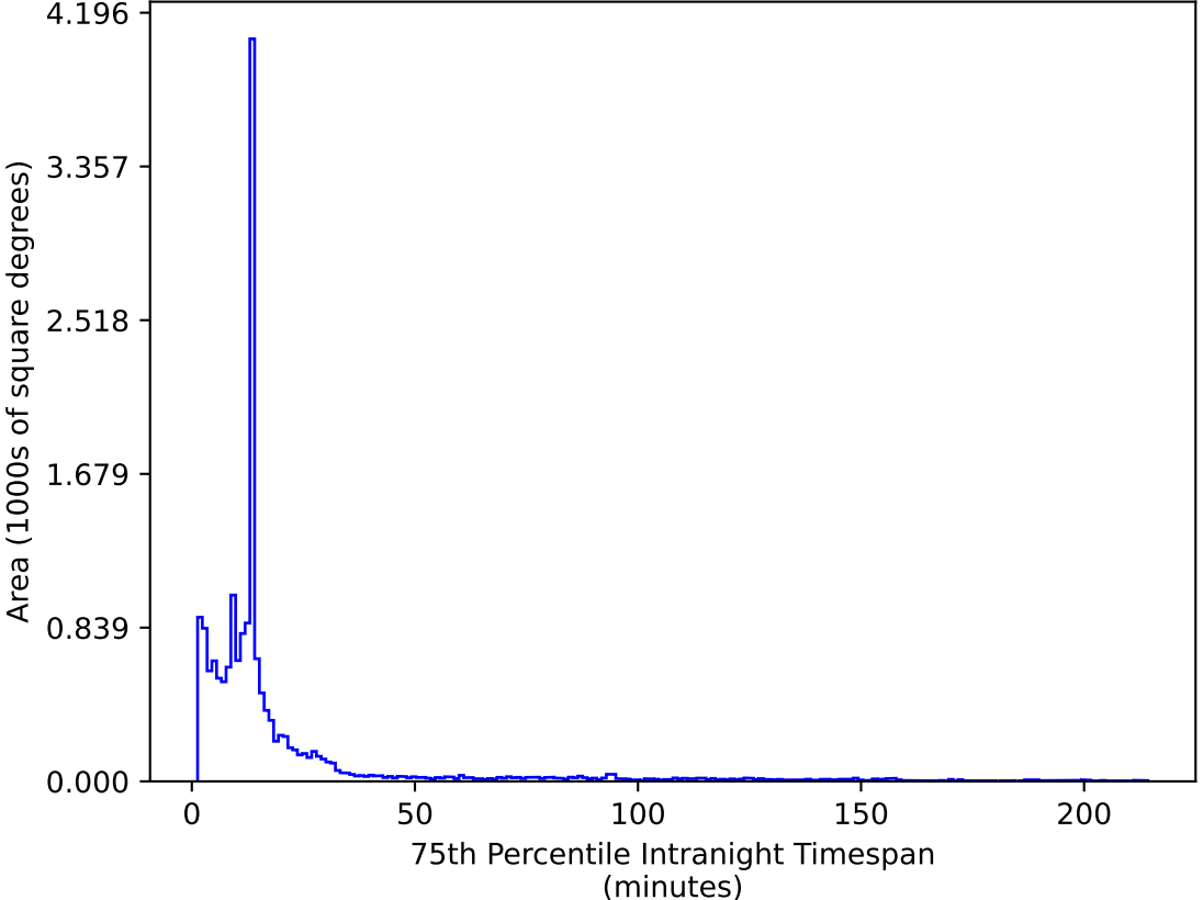
ddf_acor_sf10_lsf30_lsr20_v3.4_10yrs WFD z band: 75th Percentile Intranight Timespan
