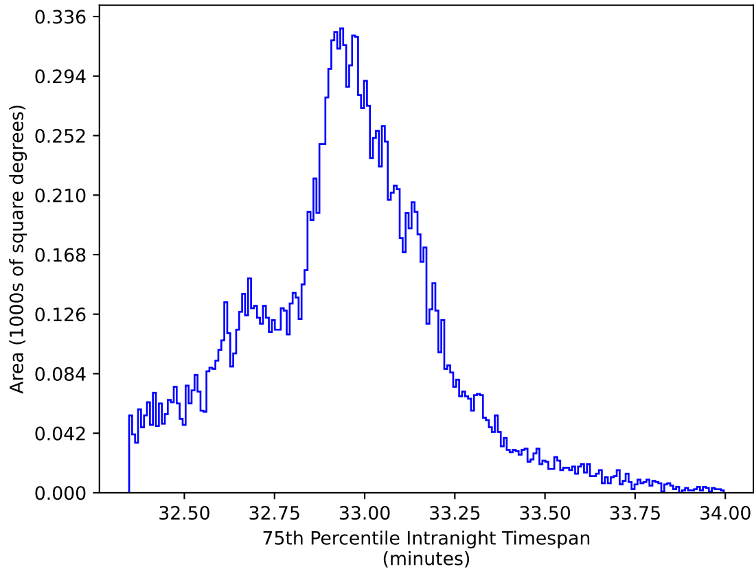
ddf_acor_sf10_lsf30_lsr20_v3.4_10yrs WFD y band: 75th Percentile Intranight Timespan
