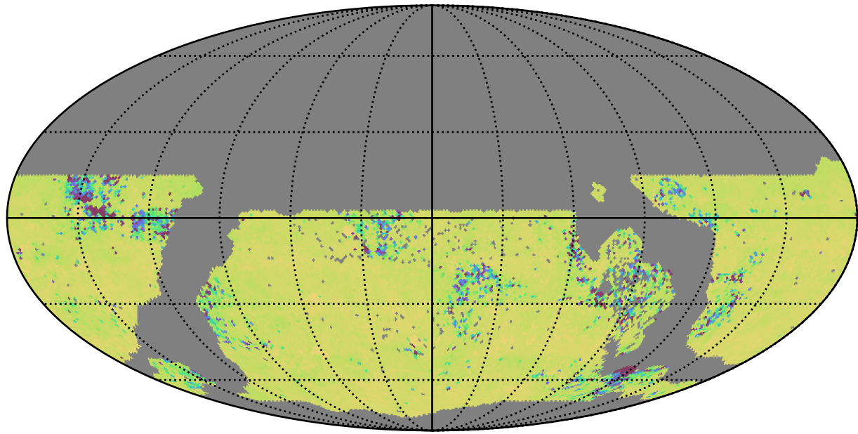
ddf_acor_sf10_lsf30_lsr20_v3.4_10yrs WFD ug bands: 75th Percentile Intranight Timespan
