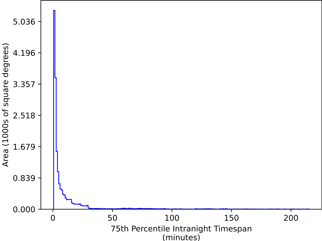
ddf_acor_sf10_lsf30_lsr20_v3.4_10yrs WFD u band: 75th Percentile Intranight Timespan
