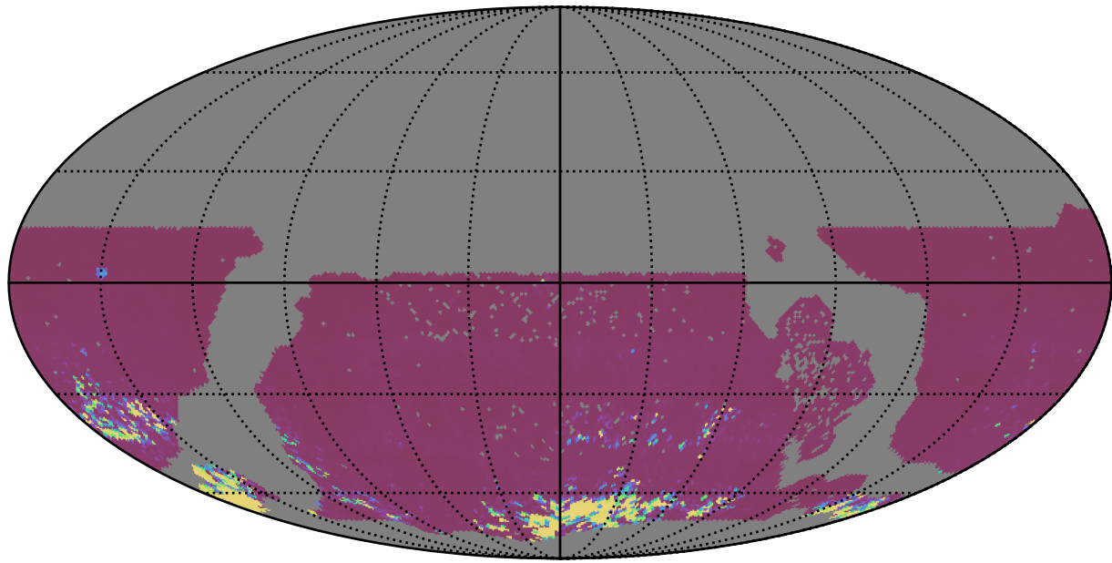
ddf_acor_sf10_lsf30_lsr20_v3.4_10yrs WFD ri bands: 75th Percentile Intranight Timespan
