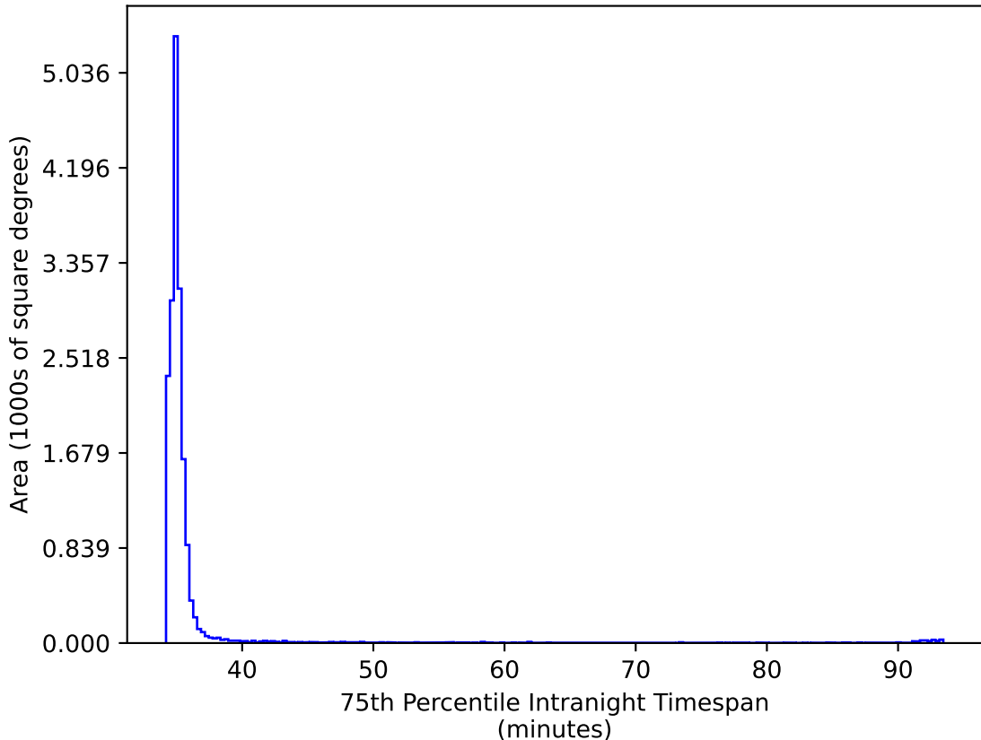
ddf_acor_sf10_lsf30_lsr20_v3.4_10yrs WFD ri bands: 75th Percentile Intranight Timespan
