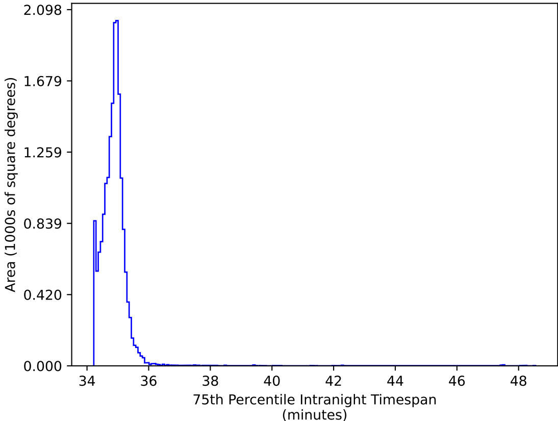
ddf_acor_sf10_lsf30_lsr20_v3.4_10yrs WFD iz bands: 75th Percentile Intranight Timespan
