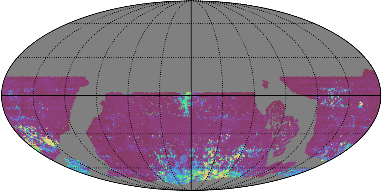
ddf_acor_sf10_lsf30_lsr20_v3.4_10yrs WFD i band: 75th Percentile Intranight Timespan
